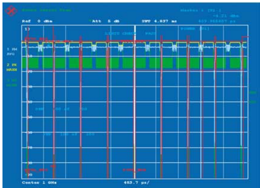
Measurement of power ramp on EDGE burst
