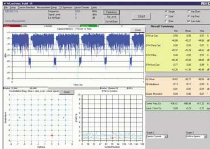
Measurement of 802.11a signal; data rate with 64QAM and simultaneous display of time characteristic, constellation diagram, EVM per OFDM symbol, and result summary with display of global error
