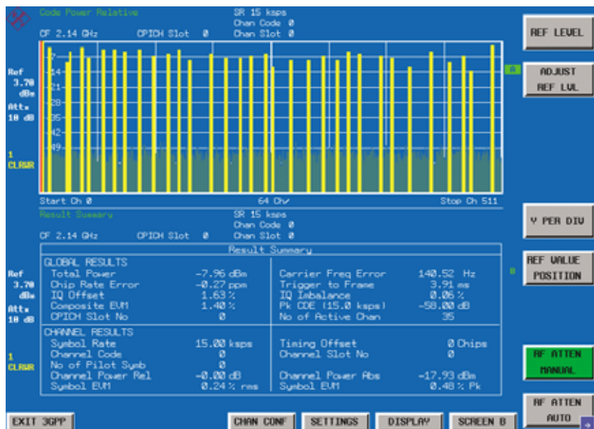
WCDMA code domain power measurement with R&S FSQ and R&S FS-K72
