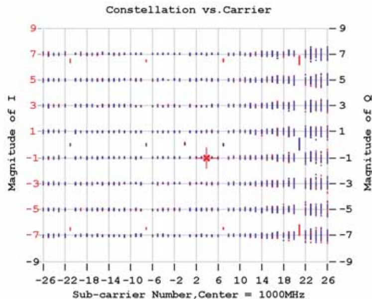
Example of adjacent-channel interference: the constellation versus carrier diagram clearly shows that the high EVM is caused by carriers on one side of the spectrum and that all steps of the 64QAM constellation are equally affected
