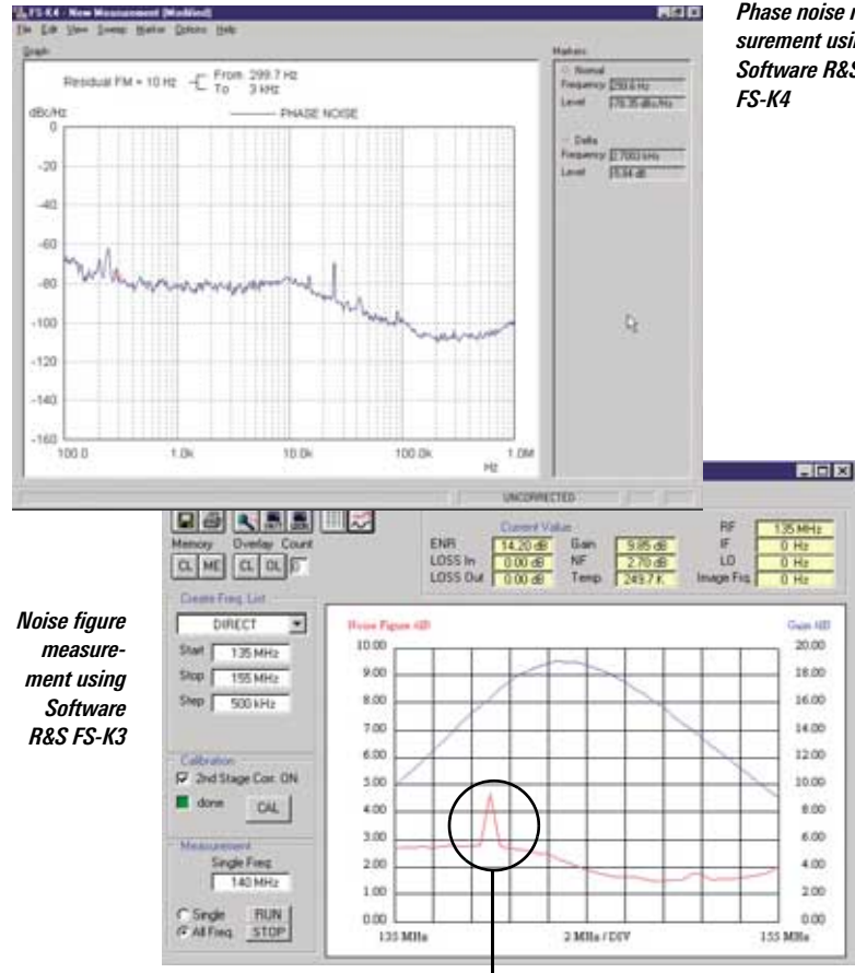
Fast and simple analysis of anomalies. The cause – spurious or RFI – can easily be traced with the basic analyzer function without additional measuring equipment.
