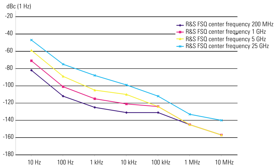
Phase noise of R&S FSQ at various center frequencies
